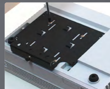
BP-500 can be mounted onto a flat surface with the FEC universal bracket.
